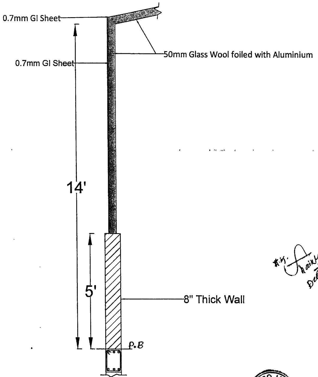
Wall Section
