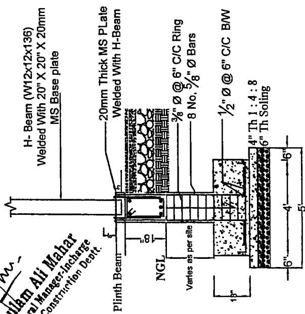
Column Foundation
